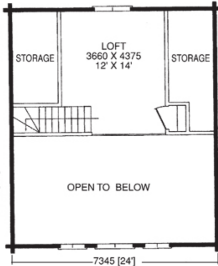
SECOND FLOOR 360 sq. ft.
