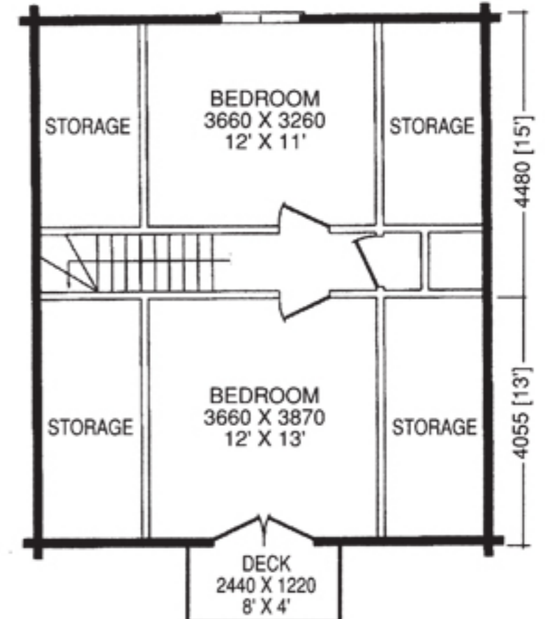
OPTIONAL SECOND FLOOR 672 sq. ft.
