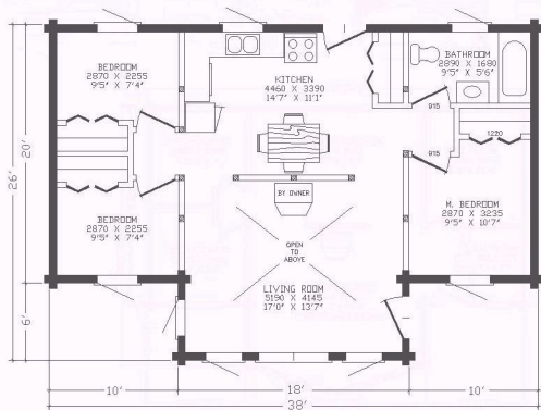
FIRST FLOOR 3 bedroom 868 sq. ft.
