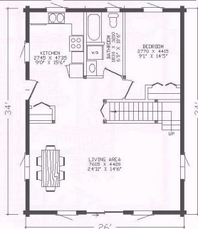
FIRST FLOOR 884 SQ.FT.
