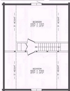
SECOND FLOOR 848 SQ.FT.
