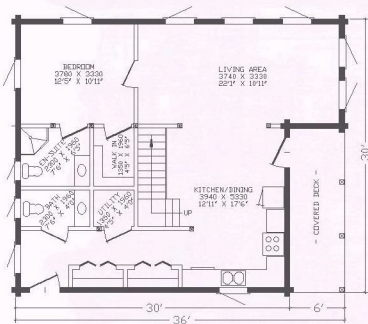
FIRST FLOOR 972 SQ.FT.
