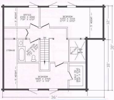
SECOND FLOOR 892 SQ.FT.
